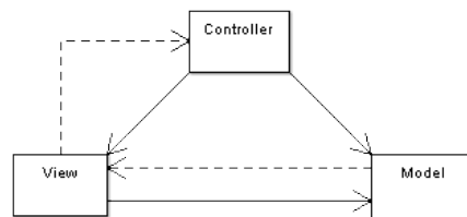
Fig. 1.2: Model-View-Controller diagram
